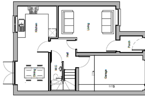
Ground Floor Plan (AS)
